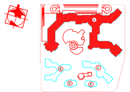
BUILDING - A FLOOR 6, LEVEL +15.00 M1:200
